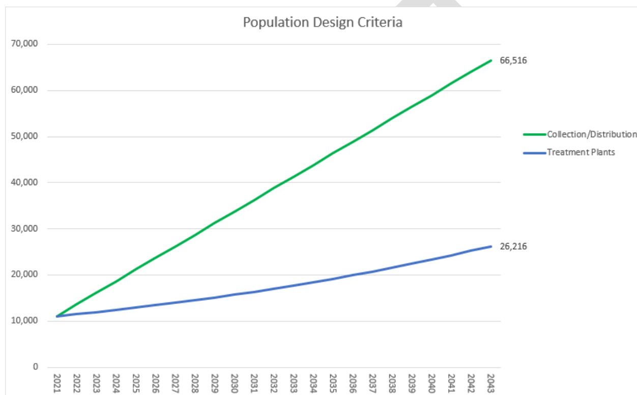
Figure 3-3: Population Projection
