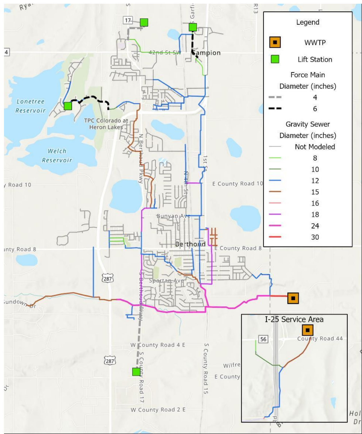
Figure 5-11: Sanitary Sewer Network
