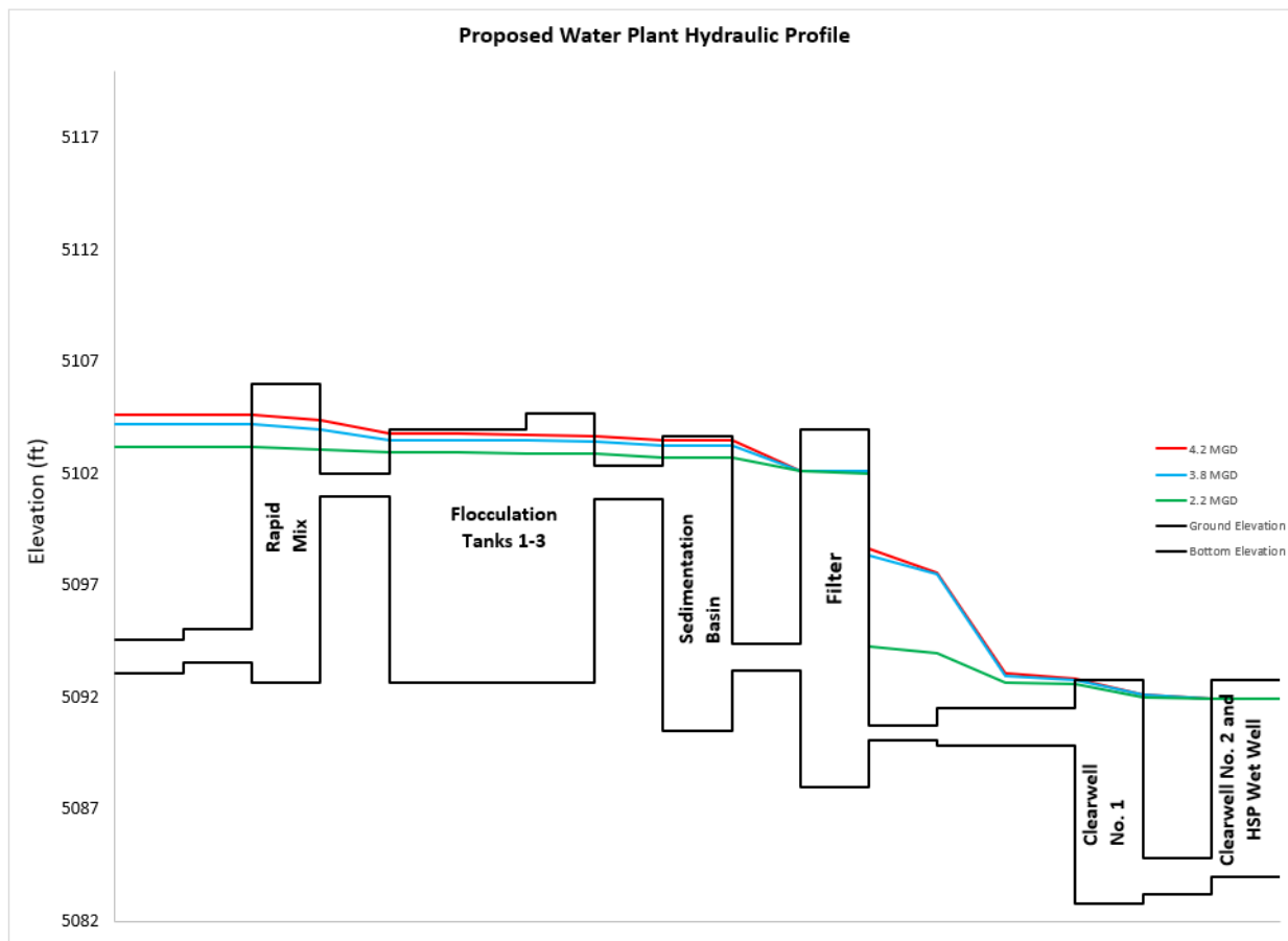
Figure 4-11: Proposed WTP Hydraulic Profile
