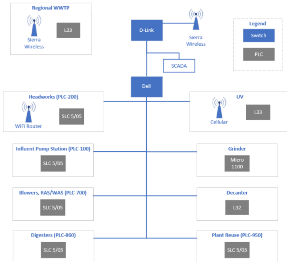
Figure 5-31: WRF-4: Existing Network Architecture
