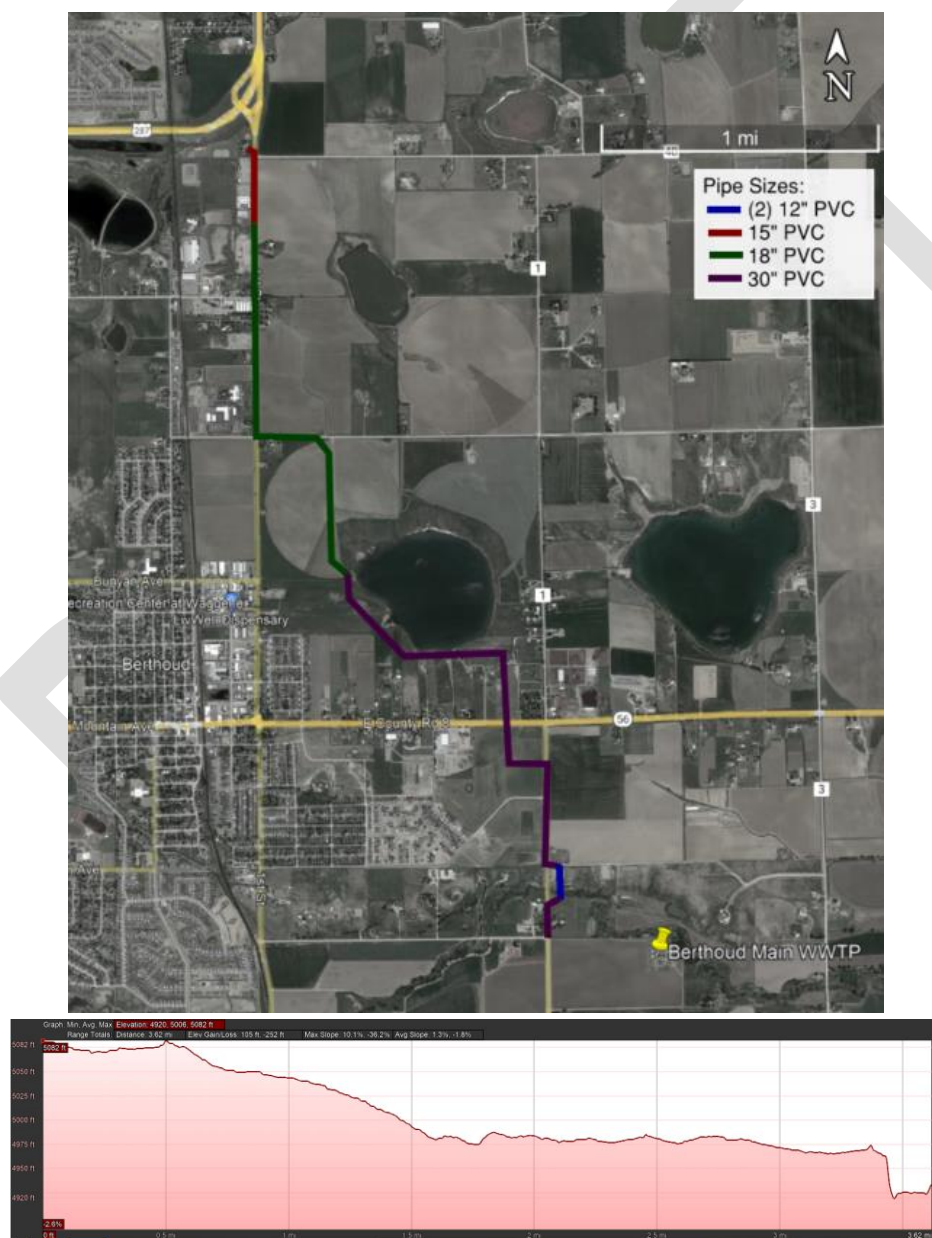
Figure 5-21: WWC-1: First Street Parallel Sewer
