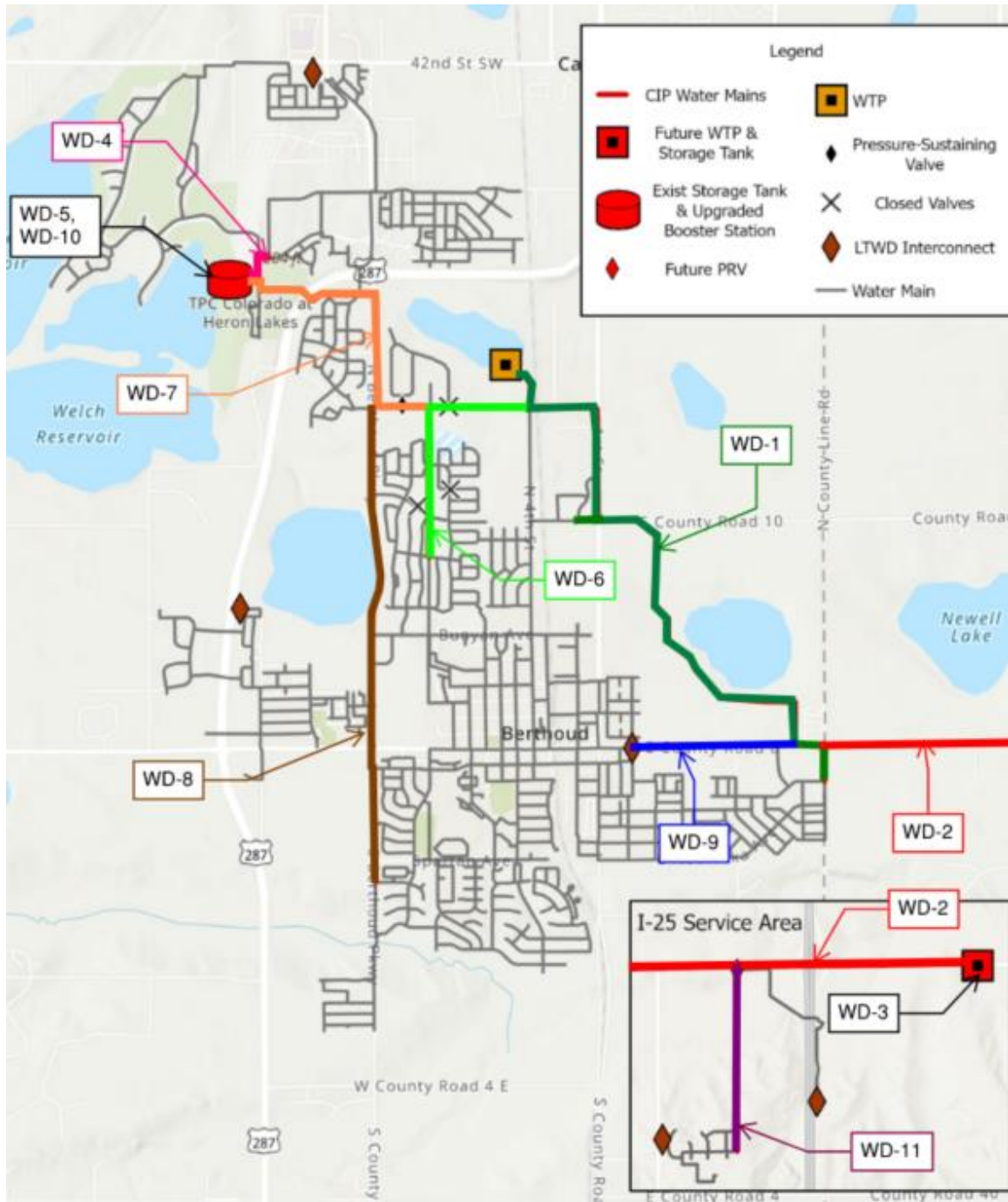
Figure 4-21: Distribution System CIP Projects
