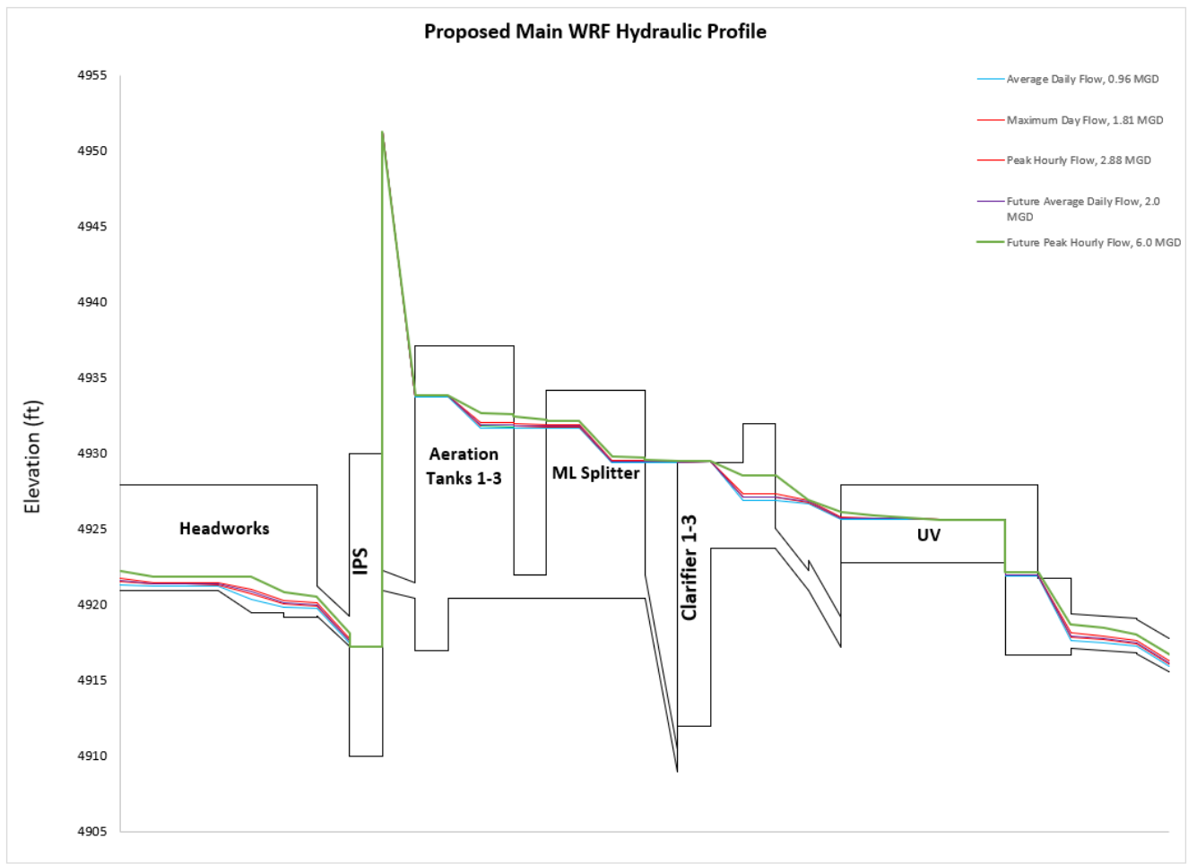
Figure 5-13: Proposed Berthoud WRF Hydraulic Profile
