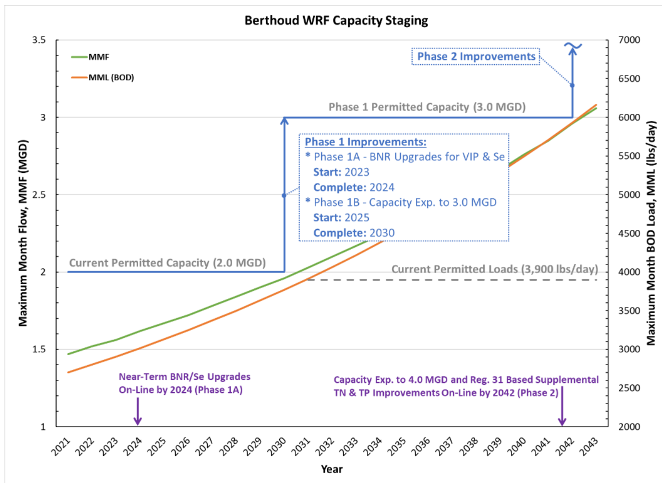
Figure 1-8: Berthoud WRF Capacity Staging Graph
