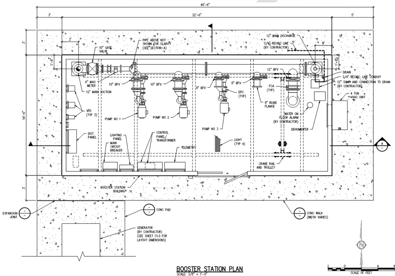
Figure 4-29: WD-5: West BPS Upgrade, Phase 1
