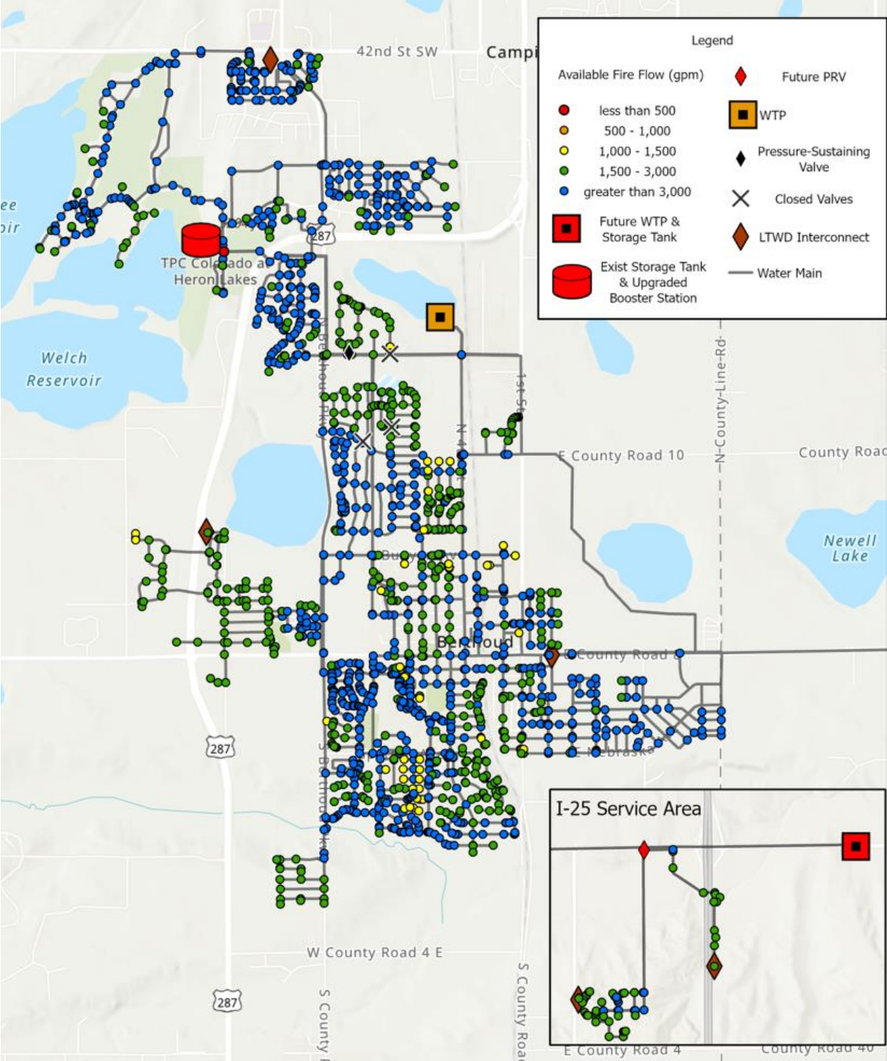
Figure 4-24: 5-Yr Improved Distribution System, Available Fire Flow
