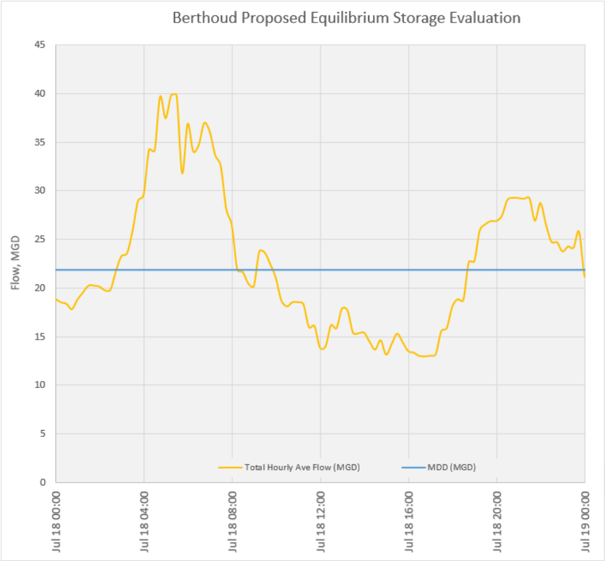
Figure 4-6: Proposed Equilibrium Storage
