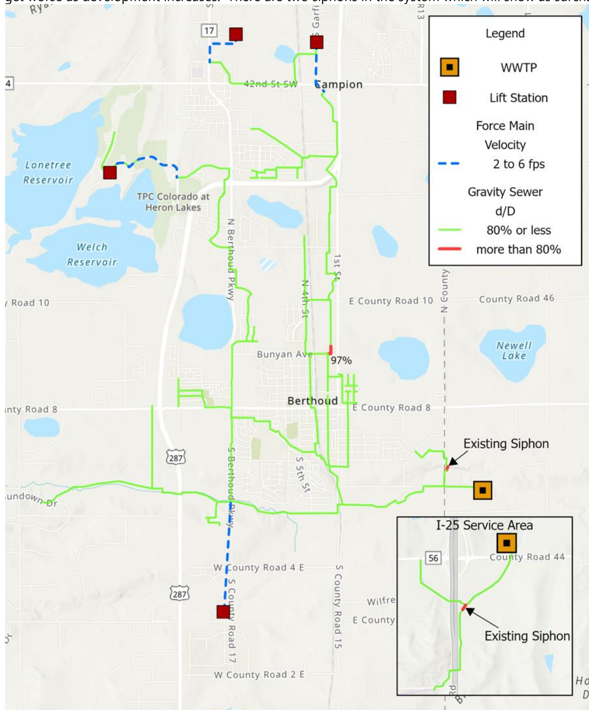
Figure 5-16: Scenario 1 – Current Conditions, Peak Flow, d/D Ratio
