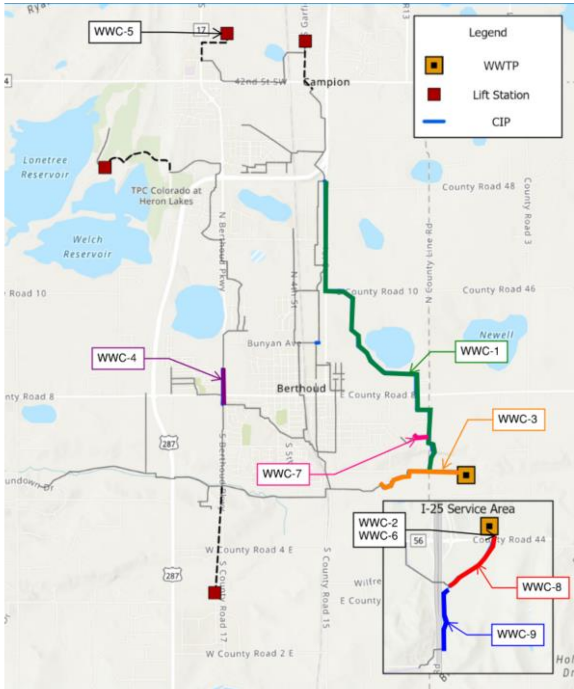
Figure 5-19: Wastewater Collection CIP Projects
