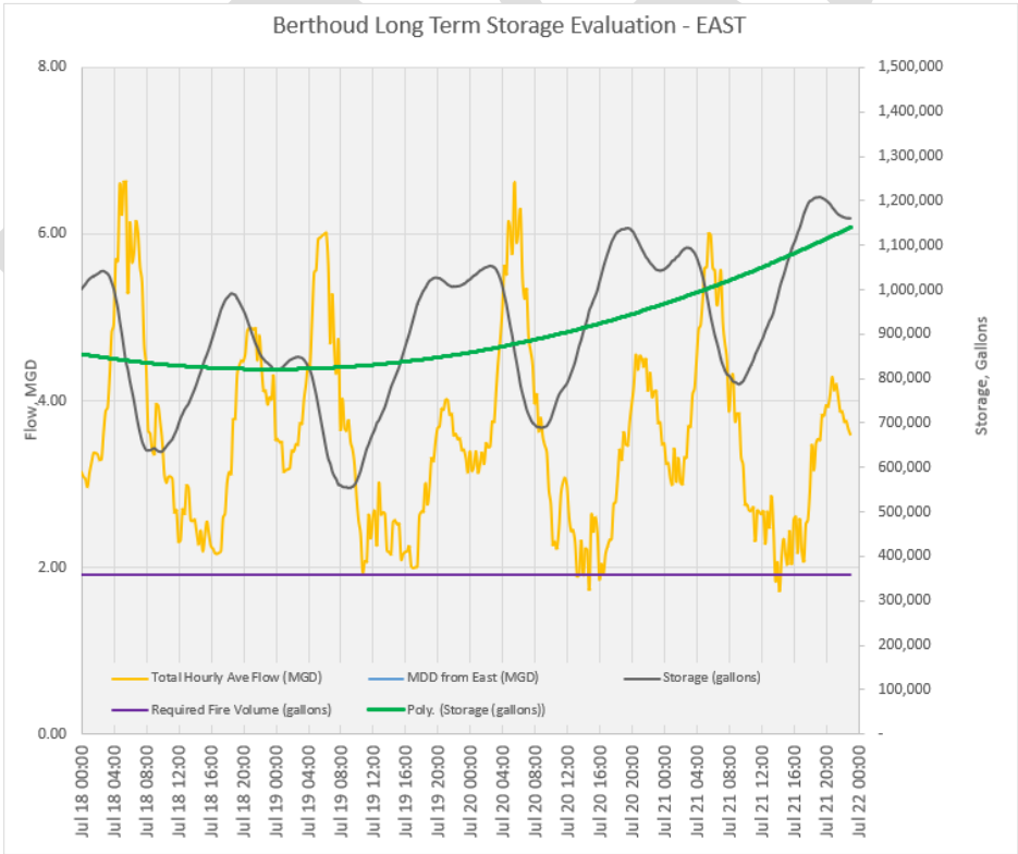
Figure 4-7: Proposed Storage 4-Day Analysis, East Zone
