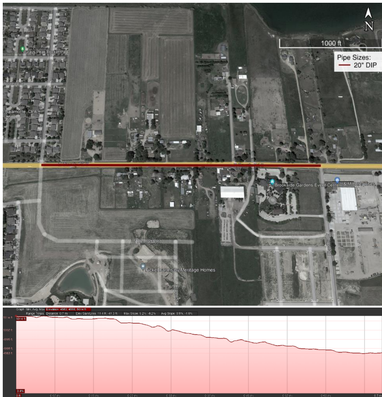
Figure 4-33: WD-9: CR 44 Transmission Main, Phase 2
