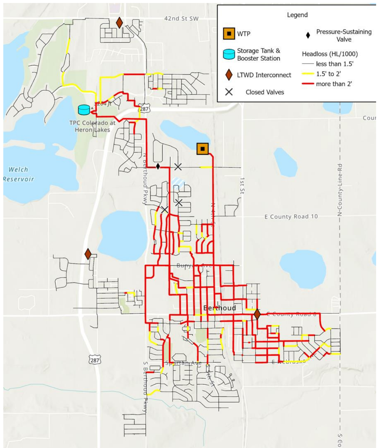
Figure 4-18: Scenario 4 – 5-Year Projection, Peak Hour Demand, Headlosses
