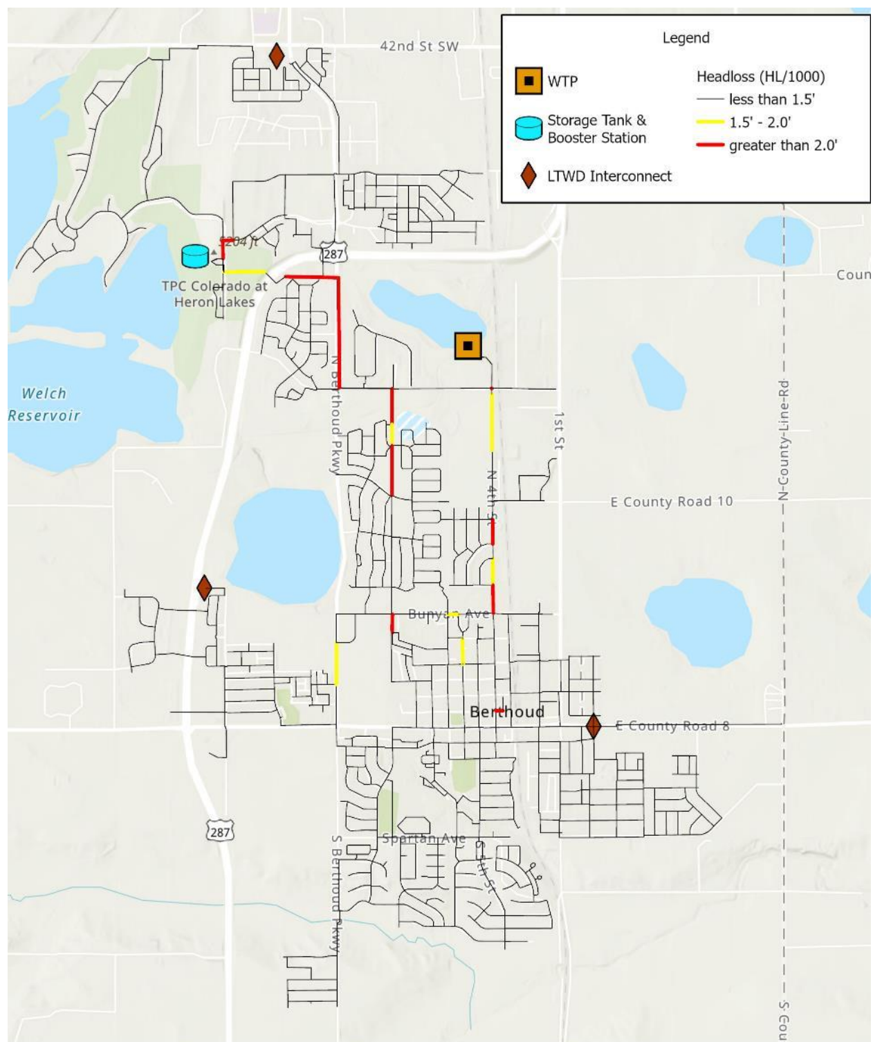
Figure 4-15: Scenario 2 – Current Conditions, Peak Hour Demand, Headlosses
