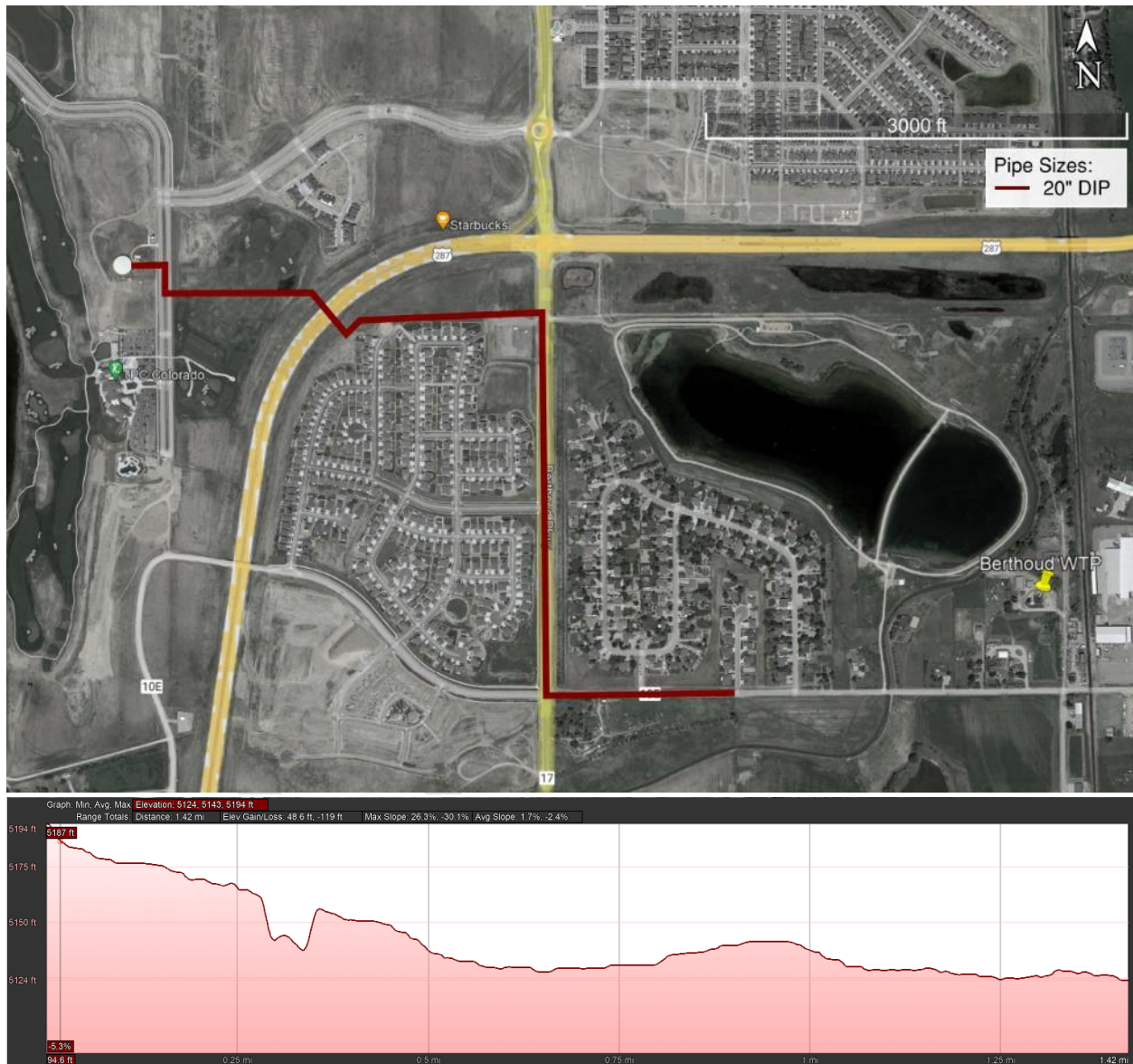
Figure 4-31: WD-7 Vantage Transmission Main
