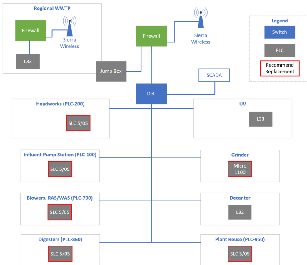
Figure 5-32: WTP-7: Recommended Network Architecture
