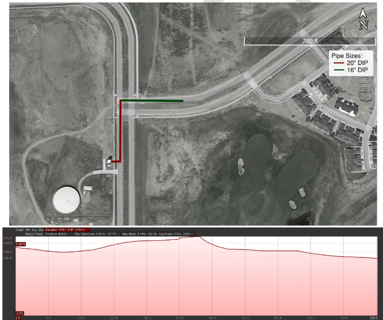
Figure 4-28: WD-4: West BPS Transmission Main
