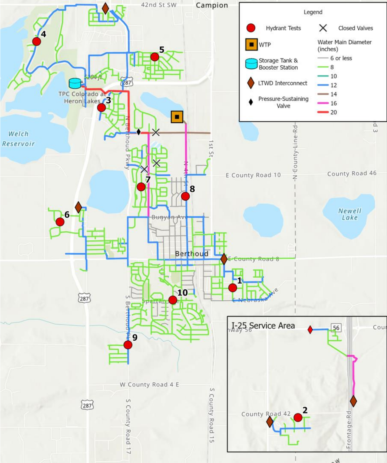
Figure 4-12: Hydrant Flow Test Locations
