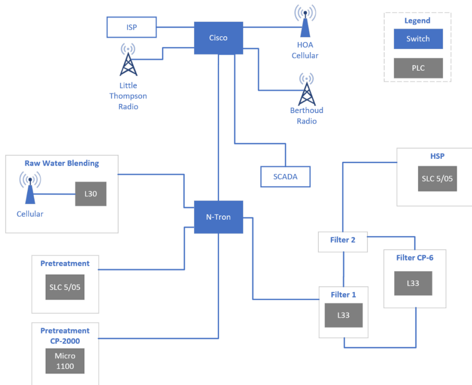
Figure 4-36: WTP-7: Existing Network Architecture
