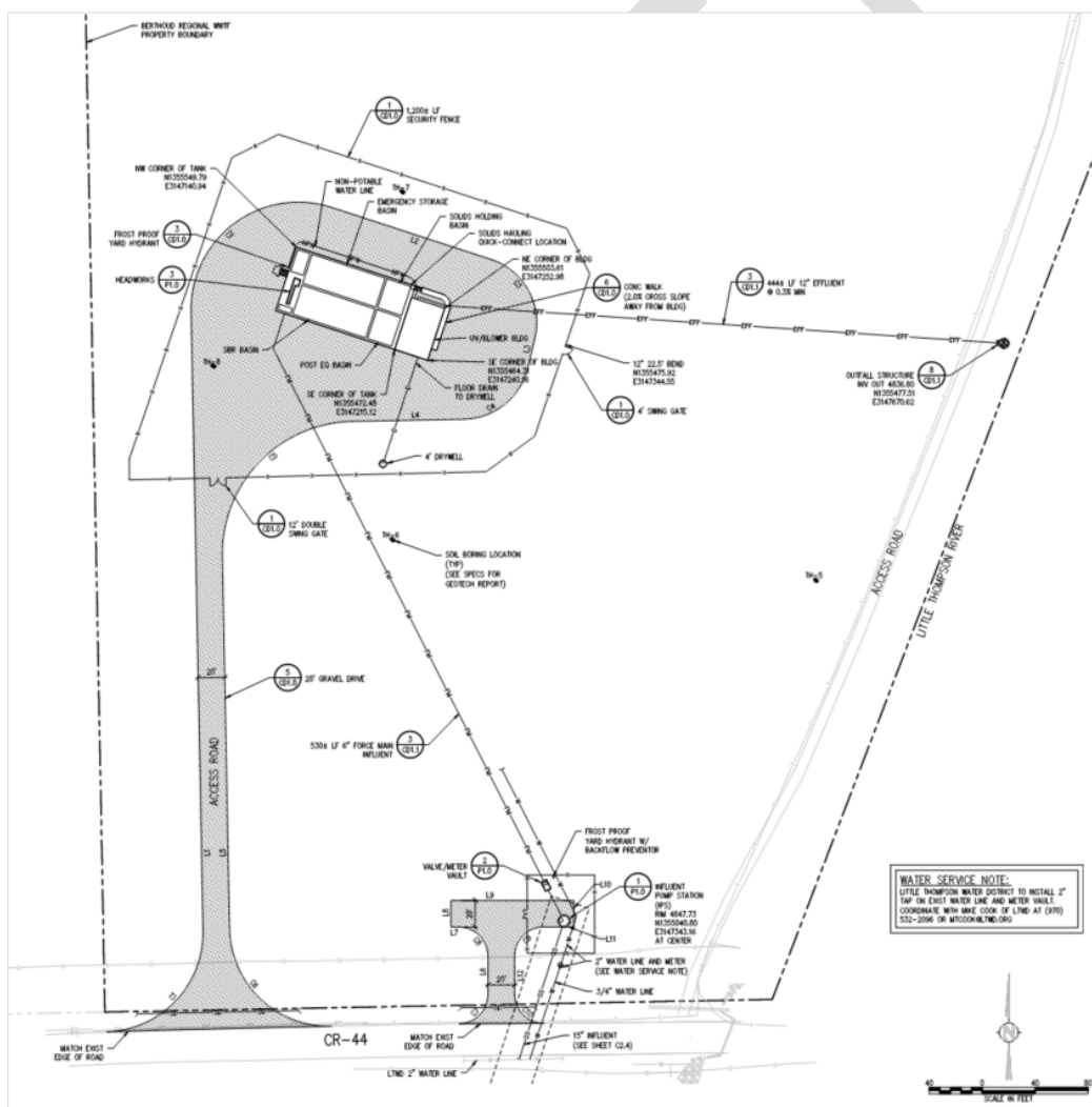
Figure 5-27: WWC-6: Regional WWTF Influent Pump Station Upgrades, Phase 1
