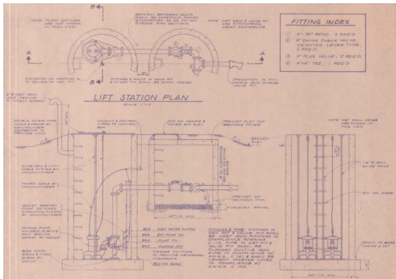
Figure 5-26: WWC-5: Bomar Lift Station Upgrades – As-Builts
