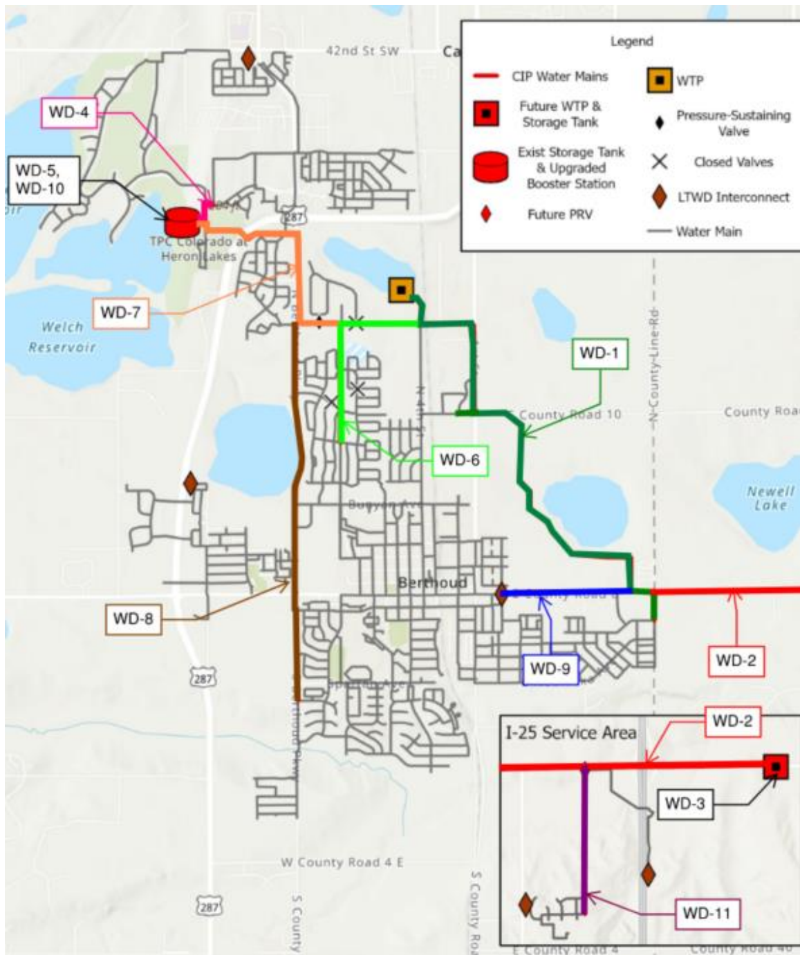
Figure 1-5: Distribution System CIP Projects
