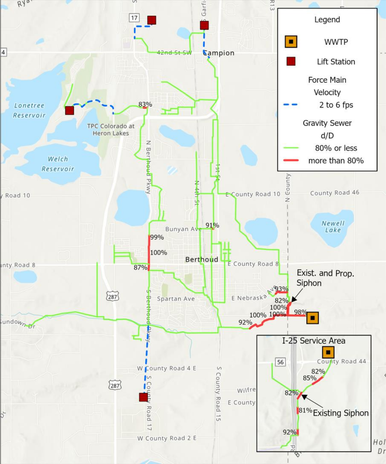
Figure 1-13: 20-Year Projection Conditions, Peak Flow, d/D Ratio
