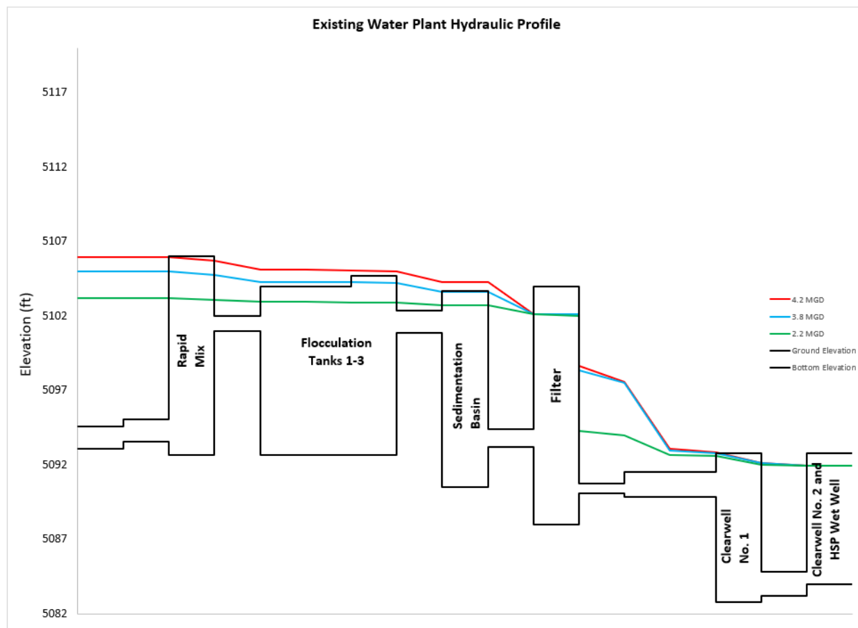
Figure 1-2: WTP Hydraulic Profile
