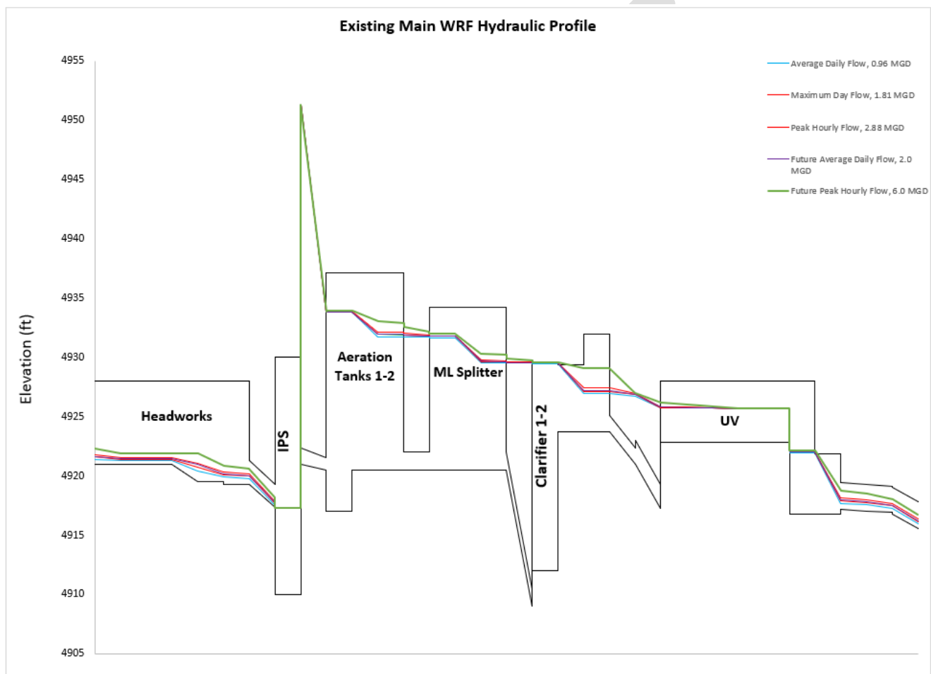
Figure 5-12: Existing Berthoud WRF Hydraulic Profile
