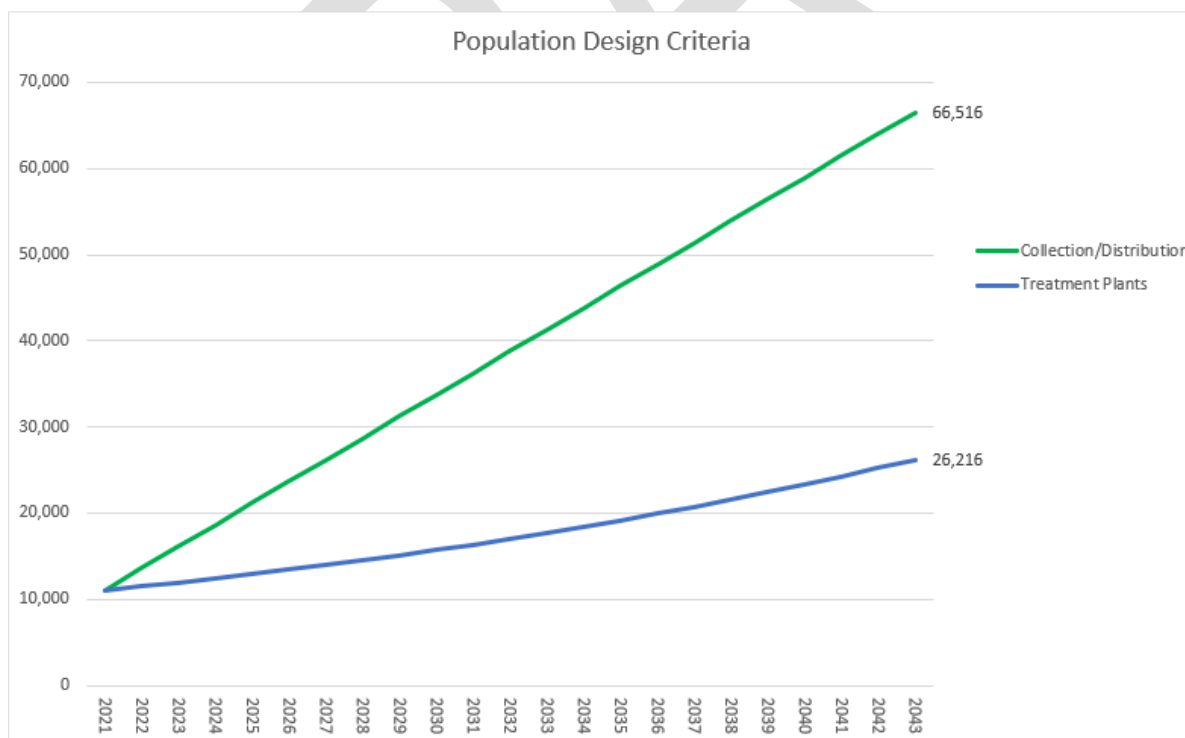
Figure 1-1: Population Projection
