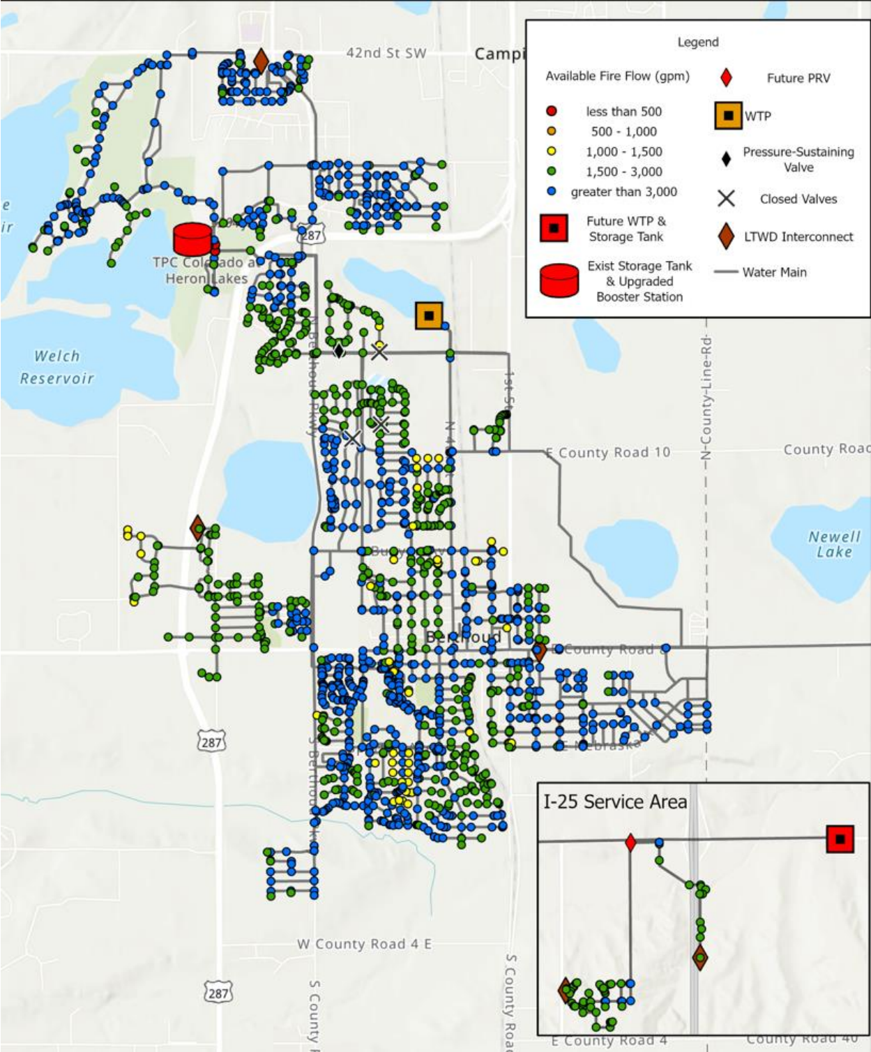
Figure 4-25: 20-Yr Improved Distribution System, Available Fire Flow
