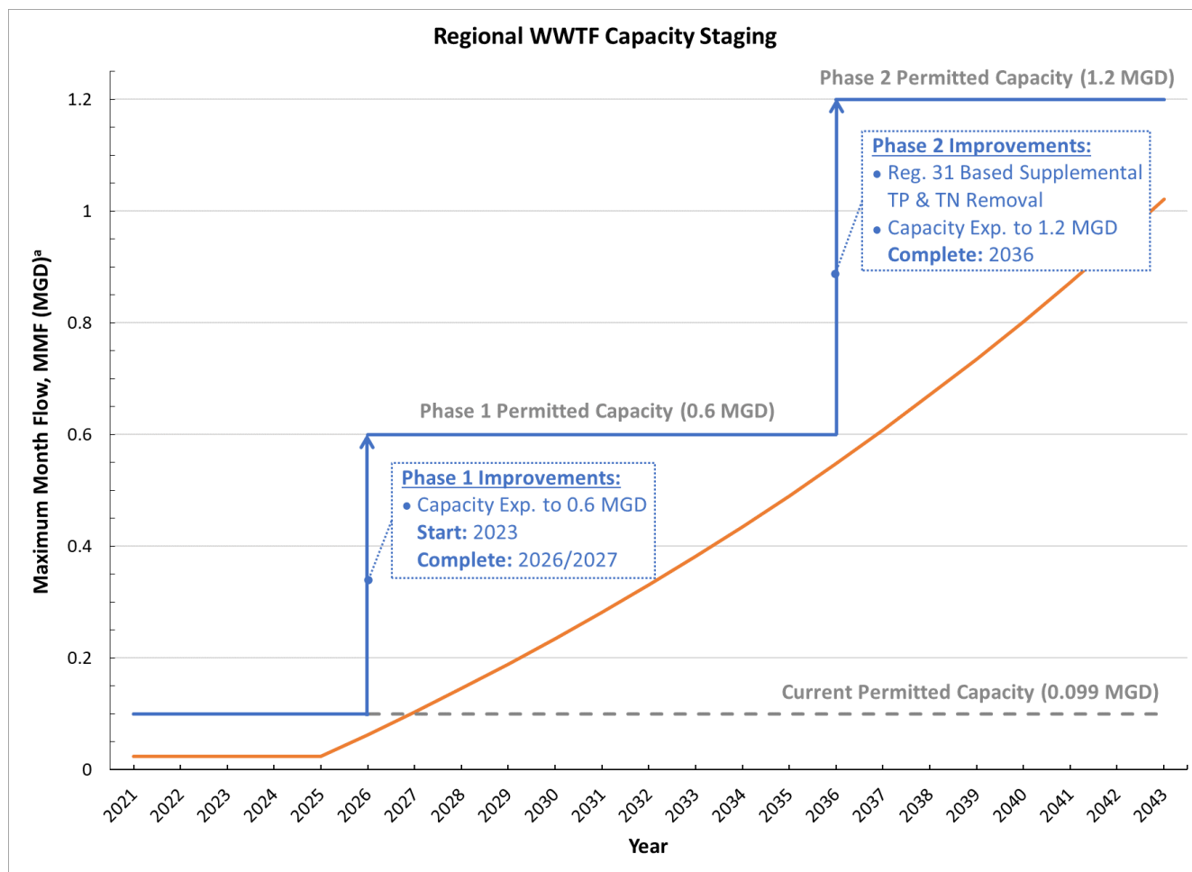
Figure 1-9: Regional WWTF Capacity Staging Graph
