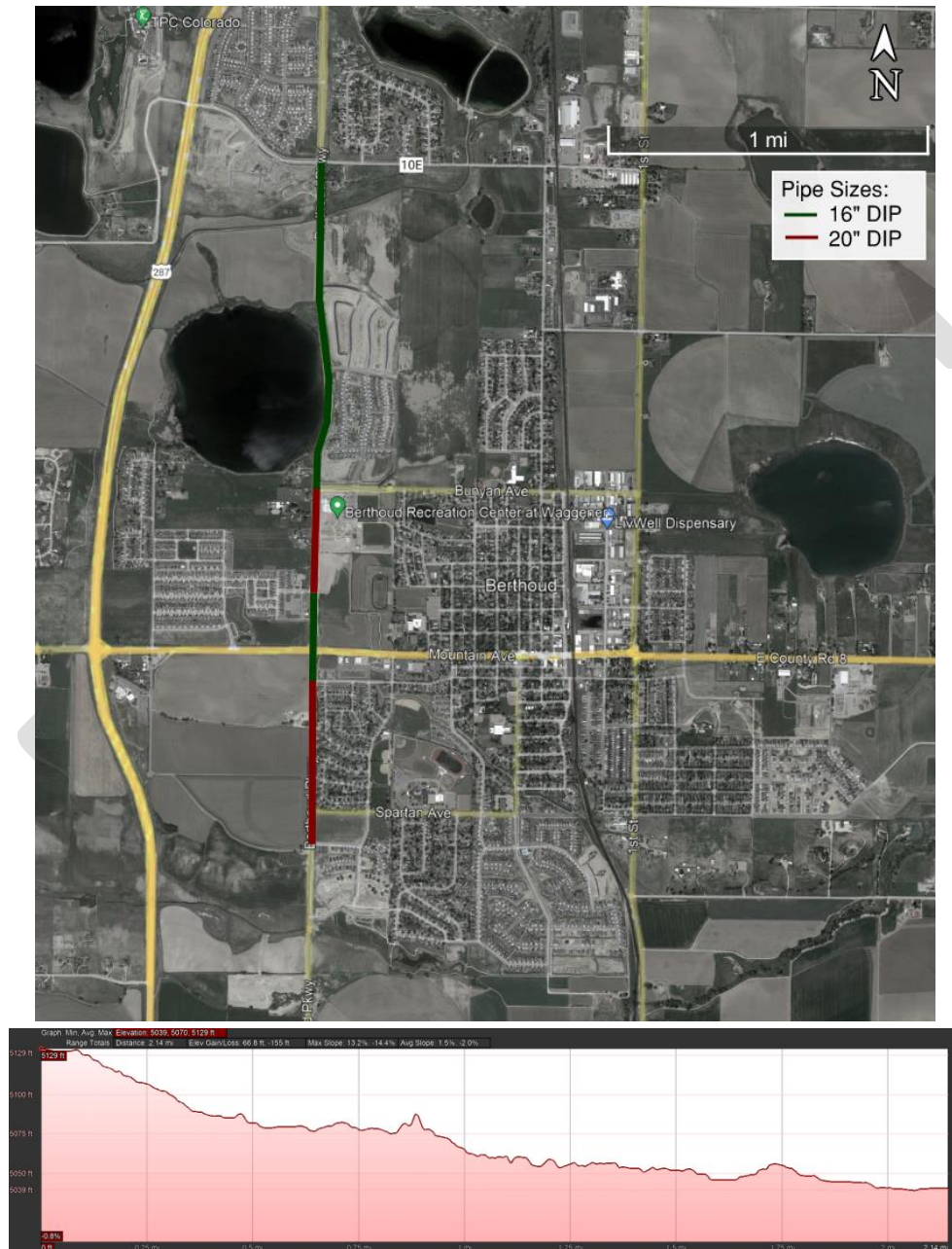
Figure 4-32: WD-8: Berthoud Parkway Transmission Main
