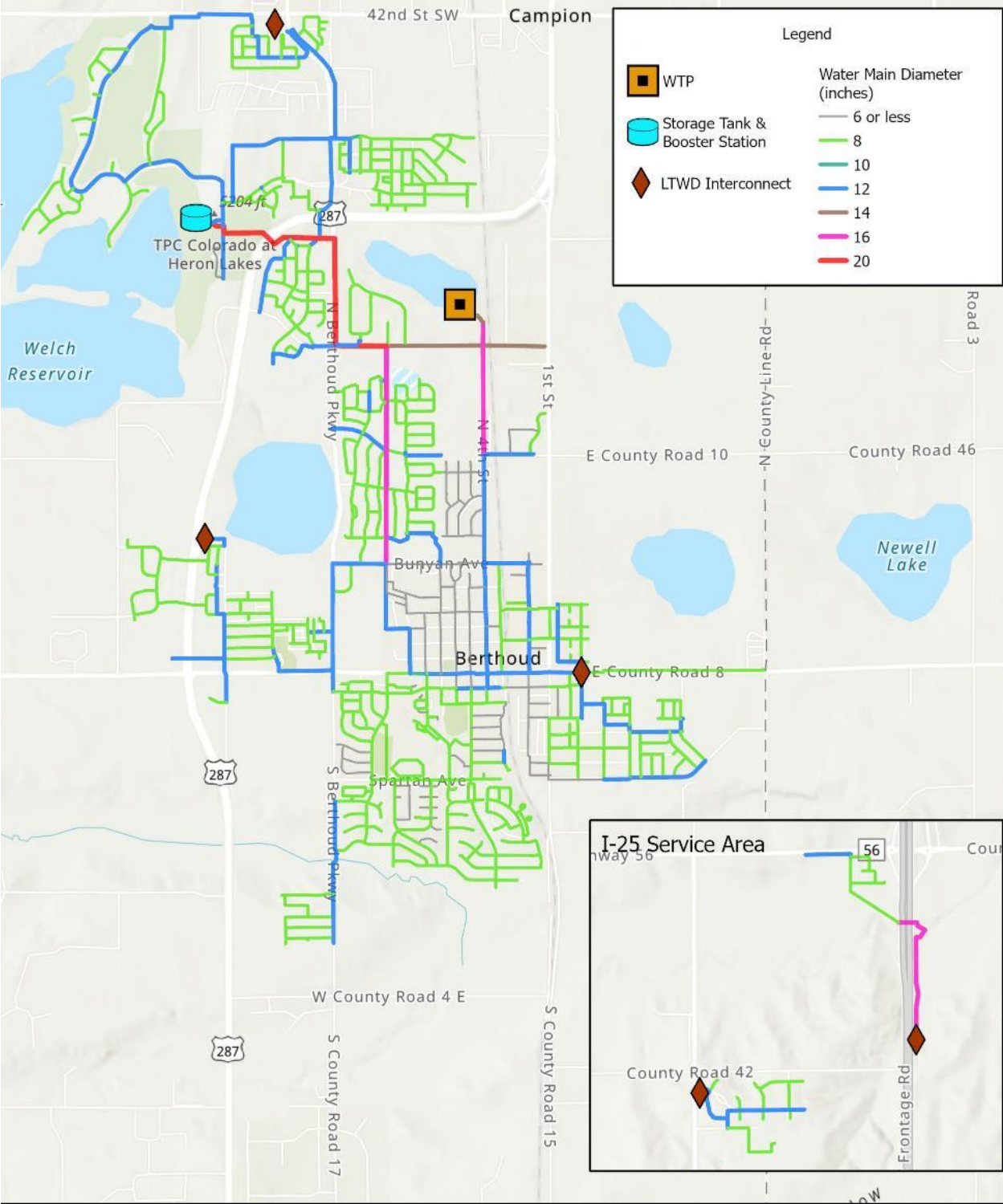
Figure 4-9: Water Main Distribution Network
