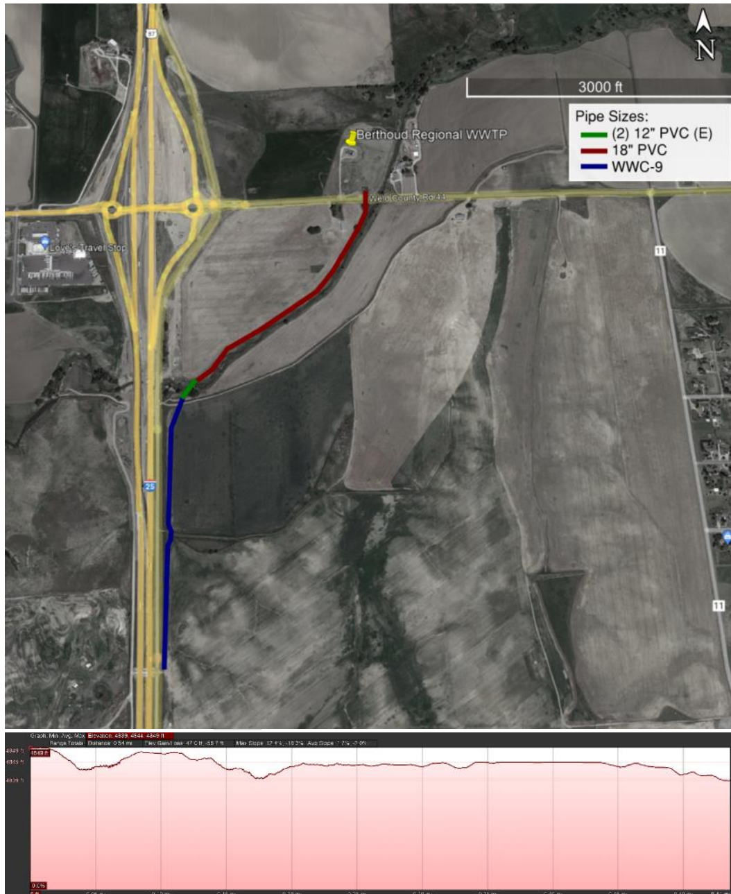
Figure 5-29: WWC-8: Turion Trunk Sewer, Phase 1
