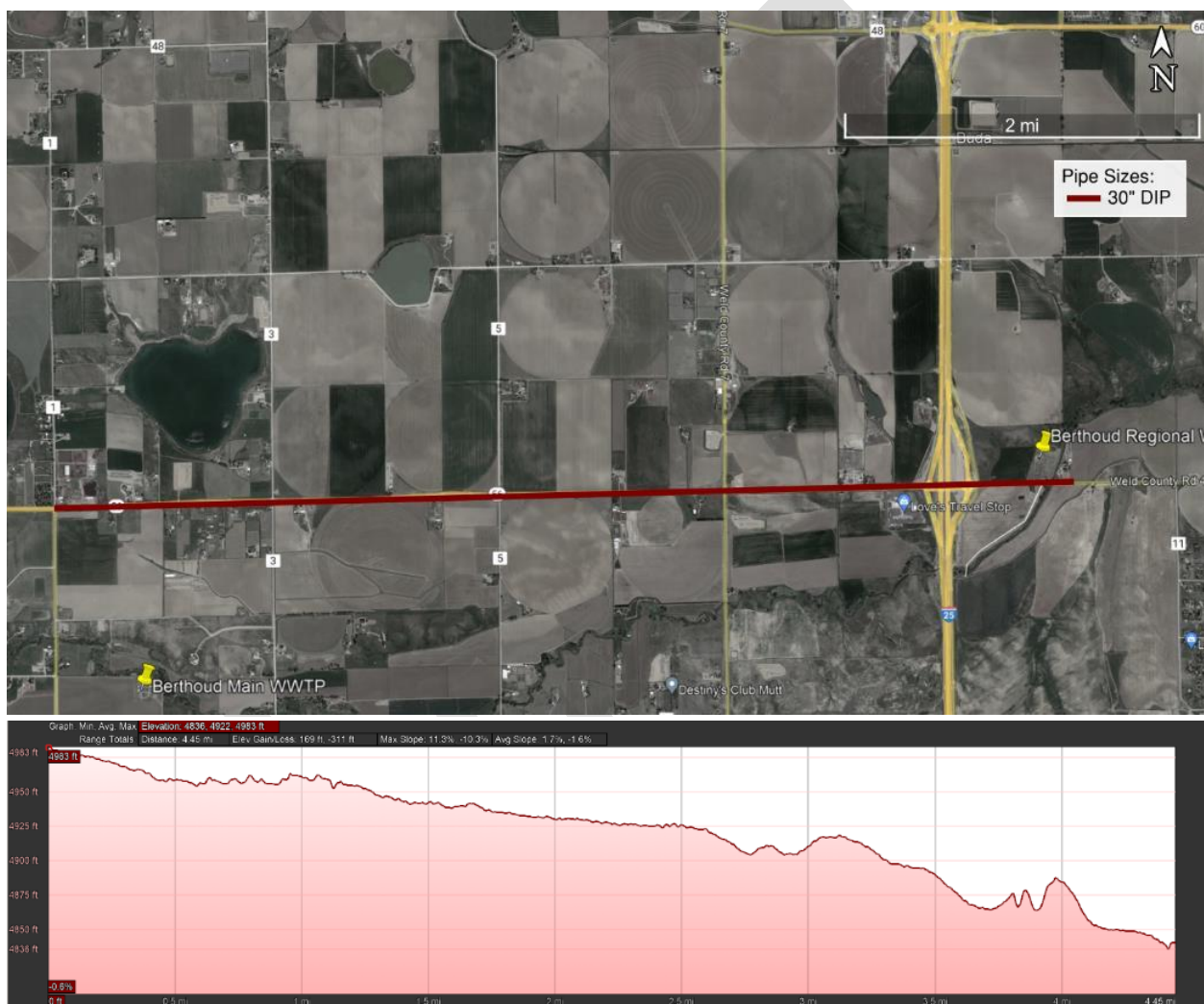
Figure 4-27: WD-2: CR 44 Transmission Main, Phase 1
