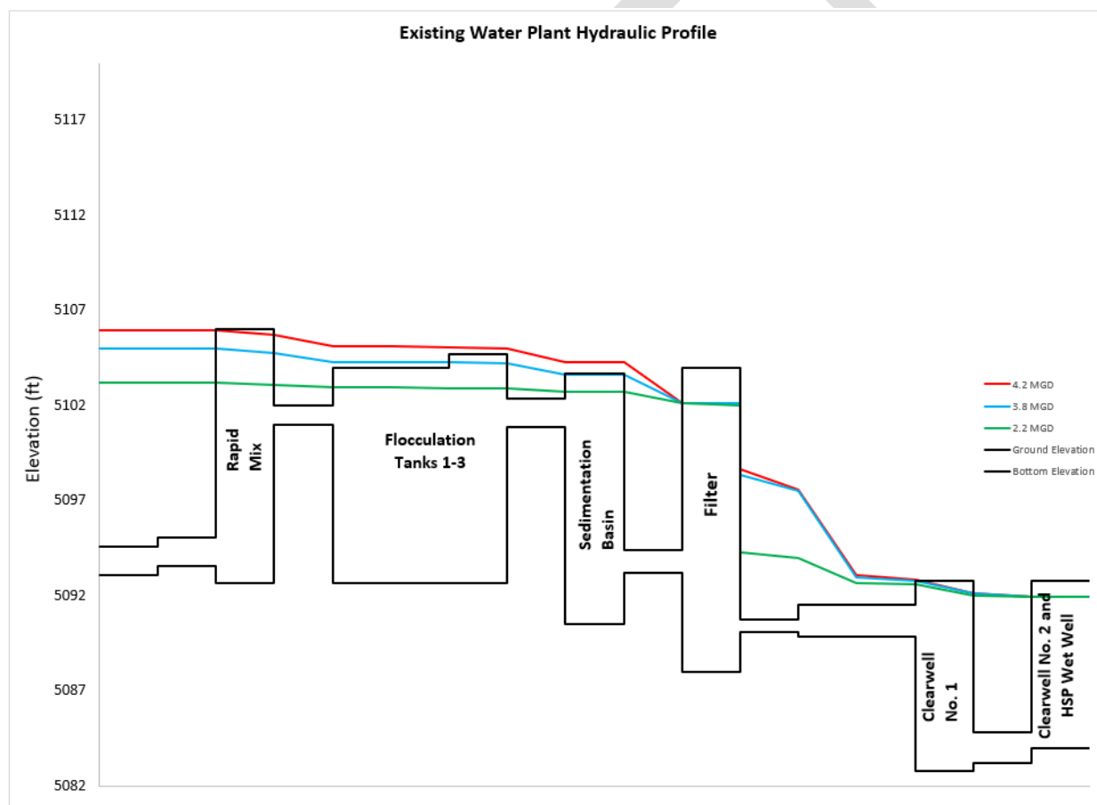
Figure 4-10: Existing WTP Hydraulic Profile
