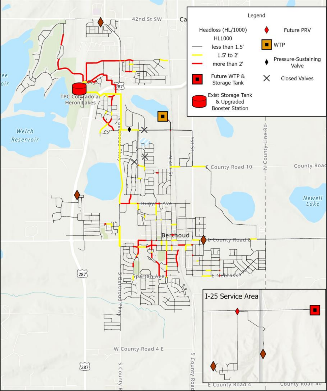
Figure 4-22: 20-Yr Improved Distribution System, Headloss
