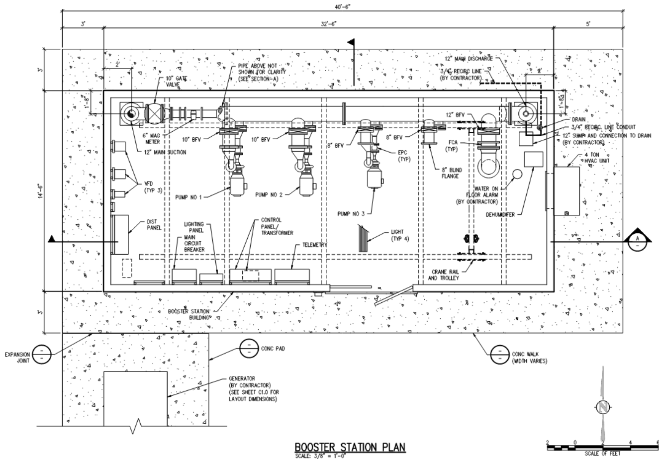
Figure 4-34: WD-10: West BPS Upgrade, Phase 2
