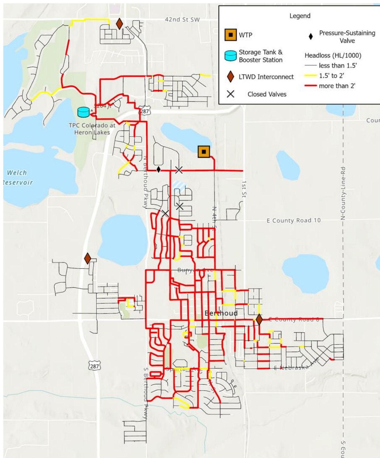
Figure 1-4: Scenario 5 – 20-Year Projection, Peak Hour Demand, Headlosses
