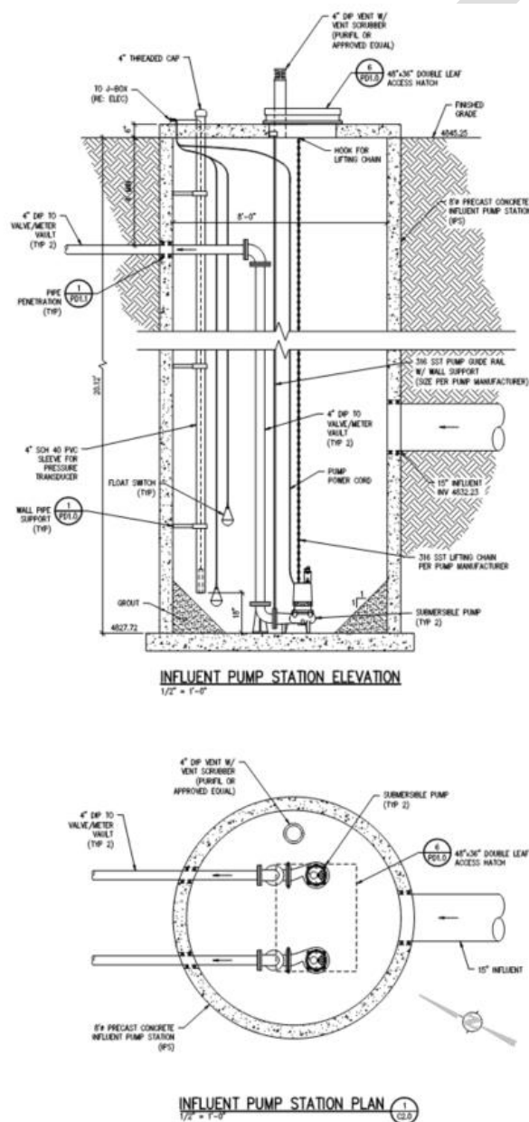
Figure 5-23: WWC-3: Regional WWTF Influent Pump Station Upgrades, Phase 1
