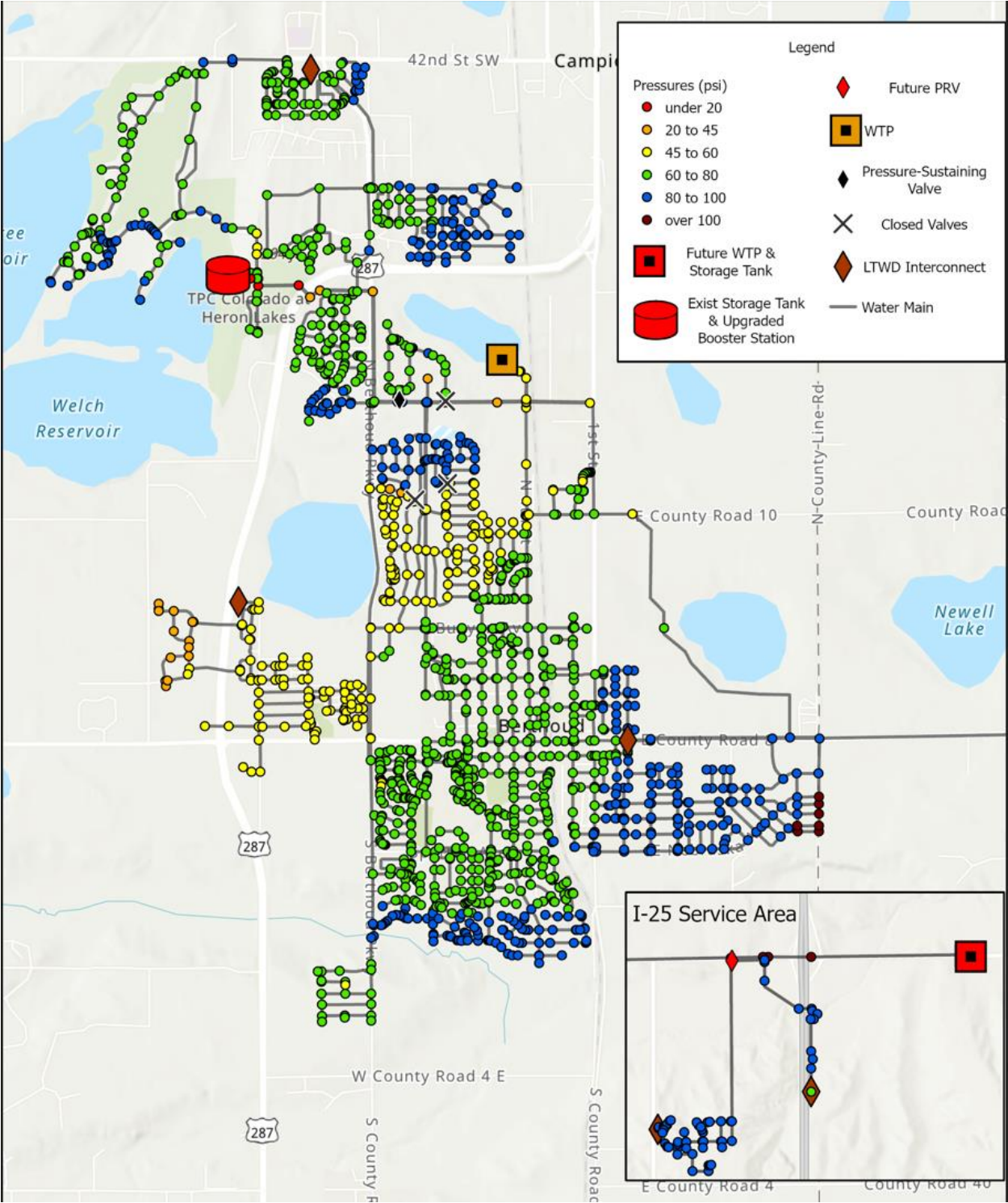
Figure 4-23: 20-Yr Improved Distribution System, Pressures
