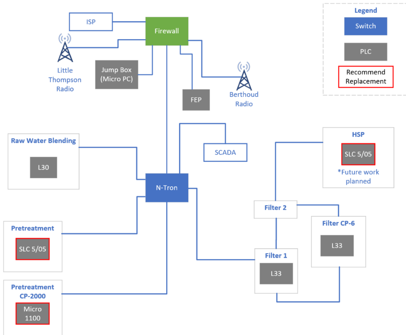
Figure 4-37: WTP-7: Recommended Network Architecture
